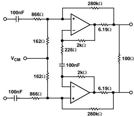
Figure 32. ADSL/ADSL2+ Circuit
